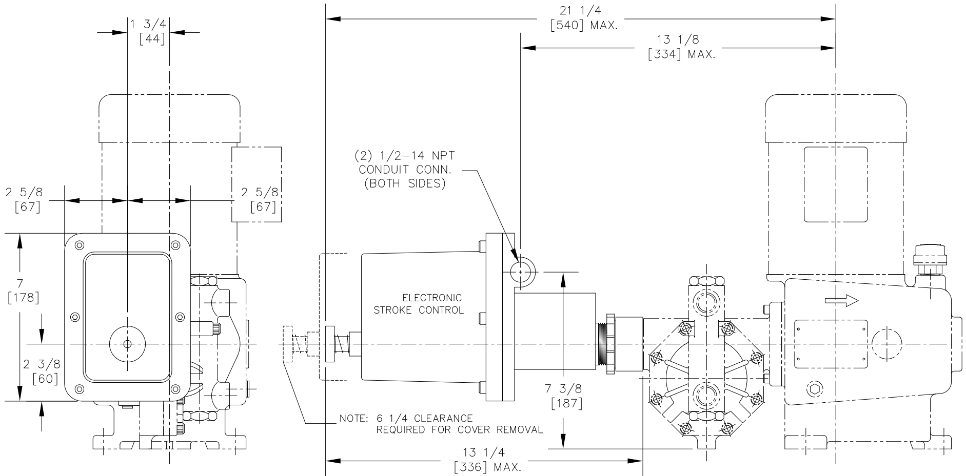
Typical Neptune dia-Pump with Electric Stroke Control
